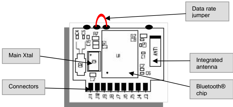
PCB top face : Bluetooth® transceiver and antenna
