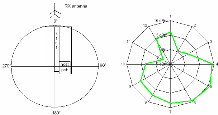
Installation TOP VIEW
