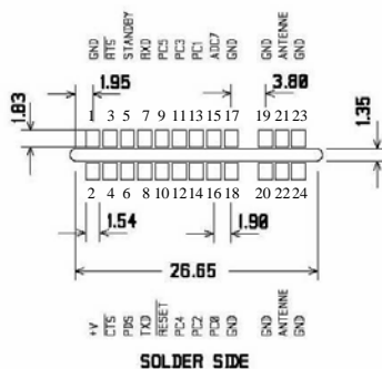
Figure 2: Plugged module mechanical feature
