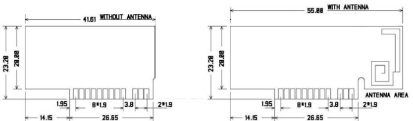
Figure 1: Two PCB formats
