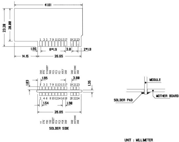
Figure 1: Plugged module mechanical feature
